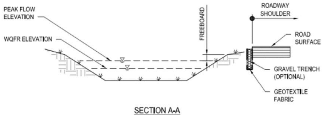
VEGETATED SWALE
